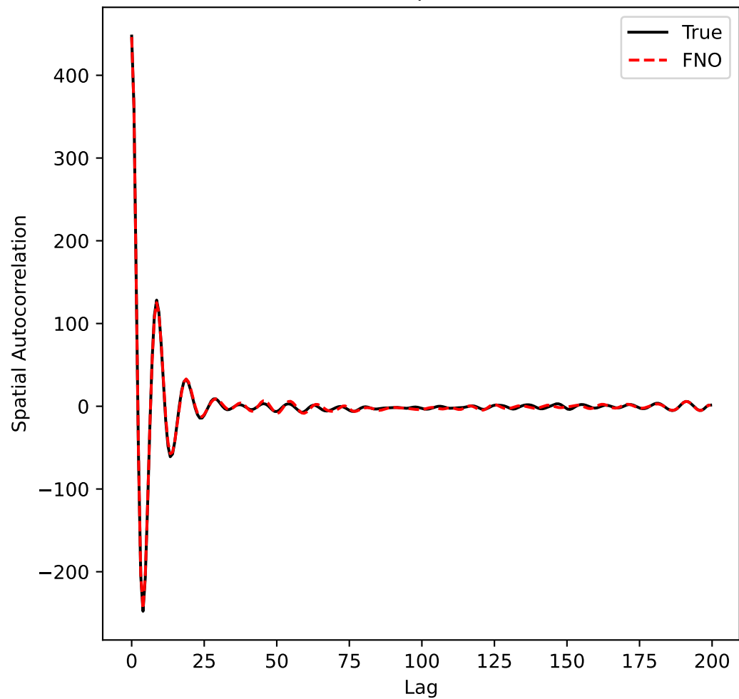
Autocorrelation Comparison with MSE = 3
