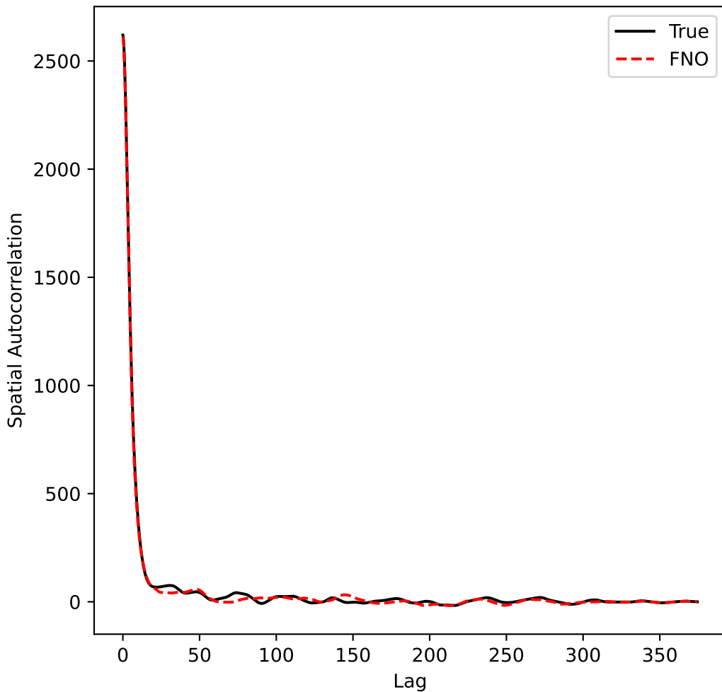
Autocorrelation Comparison with MSE = 1.8 \times 10^2
